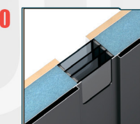
GEAM TERMOIZOLANT TRICAMERAL — GROSIME TOTALĂ 70 MM (3 STICLE x 4 MM)
